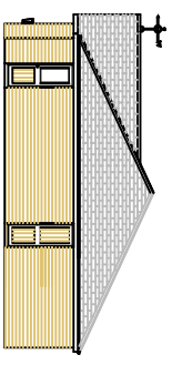
EAST END ELEVATION
